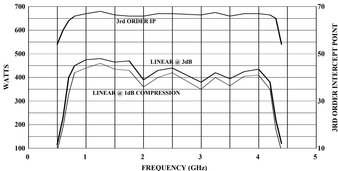
400S1G4 TYPICAL POWER OUTPUT
